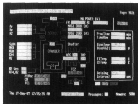
Programmable microprocessor control with ramping and data logging
