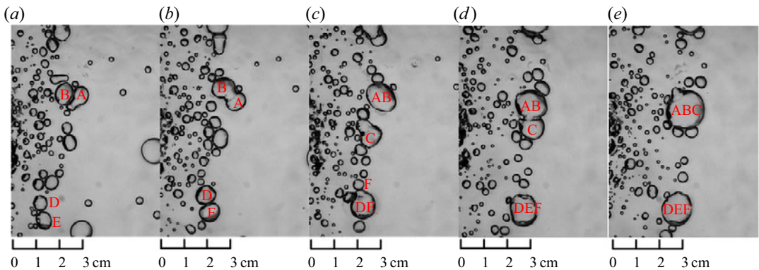
Figure 10. Backlit images of bubble clusters in the process of coalescing and bursting at C = 0 in experiment S2 for (a) t = t_0 , (b) t = t_0 + 32\Delta t , (c) t = t_0 + 50\Delta t , (d) t = t_0 + 91\Delta t and (e) t = t_0 + 108\Delta t , where \Delta t = 4 ms. Red letters (A–F) indicate original bubbles before coalescence, for reference.
