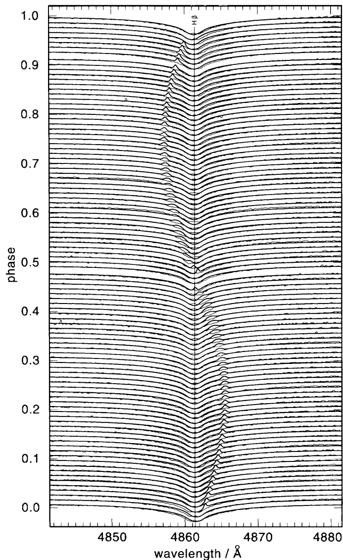
Fig. 1. Section of the UVES spectra around H\beta compared with synthetic spectra. A weak H\beta emission is used to represent the secondary's radiation.
