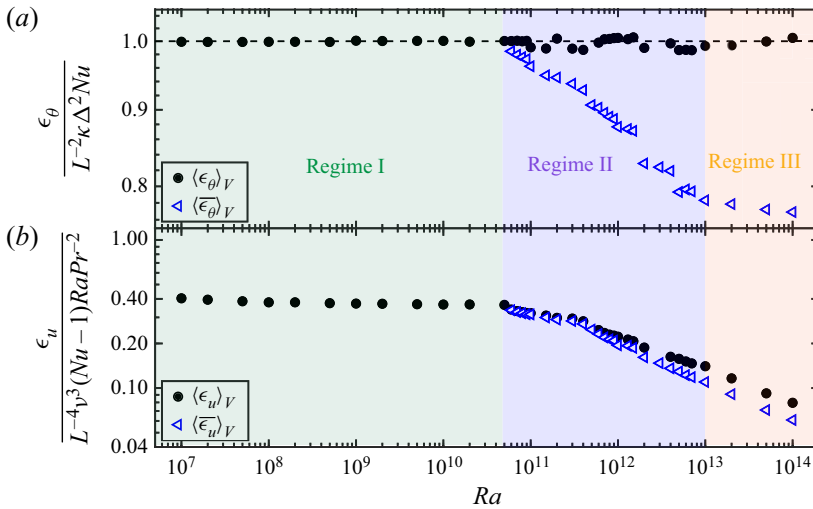
Figure 7. Normalized (a) thermal dissipation rate \langle \epsilon_\theta \rangle / (L^{-2}\kappa\Delta^2Nu) and (b) kinetic dissipation rate \langle \epsilon_u \rangle / [L^{-4}\nu^3(Nu - 1)RaPr^{-2}] as functions of Ra . The black solid circles denote the total dissipation rates while hollow triangles correspond the dissipation rates of the mean field.
