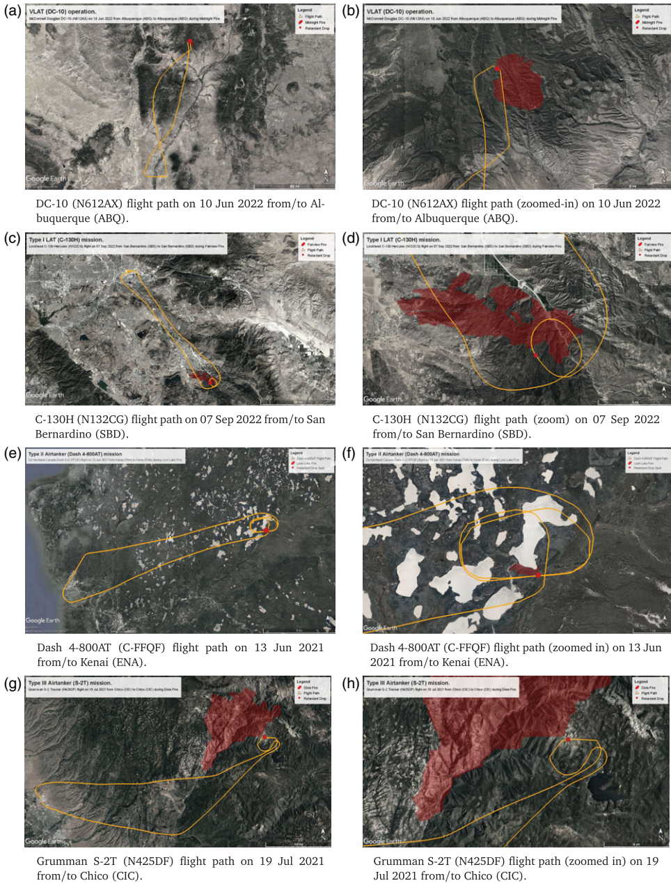
Figure 3. Flight paths of non-amphibious air tankers for selected operations; fire maps for web services such as www.wildfiretoday.com and the US National Wildfire Coordination Group ( www.nwcg.gov ).
