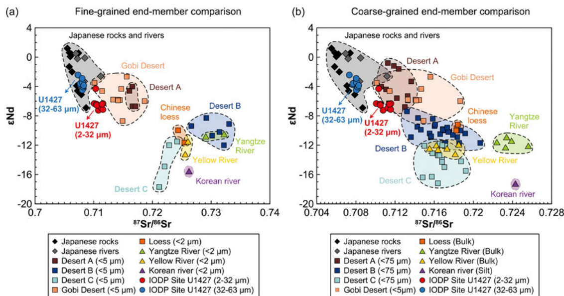
Figure 4. (Colour online) Provenance of 2–32 \mu\text{m} and 32–63 \mu\text{m} fractions from Site U1427 sediments based on the Sr-Nd isotopic composition. (a) Comparison with fine-grained end-members of potential source areas. (b) Comparison with coarse-grained end-members of potential source areas. Data sources: Japanese rivers (Goldstein & Jacobsen, 1988; Shen et al. 2017), Japanese rocks (Kagami et al. 1992), Deserts A, B and C (Chen et al. 2007), Gobi Desert (Biscaye et al. 1997; Zhao et al. 2015), Chinese loess (Chen et al. 2007; Zhao et al. 2017), Yangtze River (Meng et al. 2008; Yang et al. 2007; Zhao et al. 2017), Yellow River (Hu et al. 2012; Meng et al. 2008; Zhao et al. 2017), Korean river (Lee et al. 2008; Lim et al. 2015).
