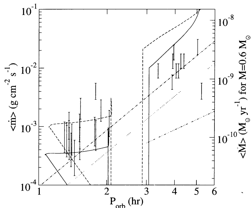
Fig. 1. Values for the time averaged accretion rate per WD surface area, \langle \dot{m} \rangle \equiv \langle \dot{M} \rangle / 4\pi R^2 , derived from the T_{\text{eff}} measurements in the table appearing in Winter & Sion (2003). The ranges indicated for each measurement are those allowed for 0.05M_{\text{ign}} < M_{\text{acc}} < 0.95M_{\text{ign}} and 0.6M_{\odot} < M < 1.2M_{\odot} . The curves show the \langle \dot{m} \rangle predicted by Howell, Nelson, & Rappaport (2001) for M = 0.7M_{\odot} (solid line) and M = 1.1M_{\odot} (dashed line), Andronov et al. (2003) (dot-dot-dashed line), and Patterson's (1984) relation deduced from CV observations for M = 0.6M_{\odot} (dotted line) and 1.0M_{\odot} (dashed line). The right hand scale gives \langle \dot{M} \rangle_{0.6} , the corresponding accretion rate if R is that for M = 0.6M_{\odot} . At the same \langle \dot{m} \rangle , \langle \dot{M} \rangle_{1.0} = 0.4\langle \dot{M} \rangle_{0.6} .
