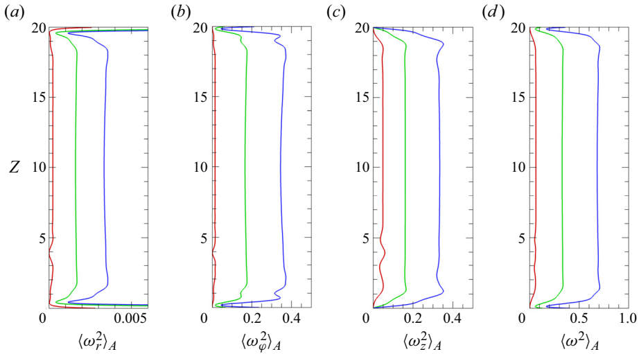
Figure 7. Profiles of the (r, \varphi) -averaged entrophy ( \langle \omega^2 \rangle_A ) and the components ( \langle \omega_i^2 \rangle_A ) for three values of V_E (red, V_E = 500 ; green, V_E = 600 ; blue, V_E = 700 ). Here, \langle X \rangle_A denotes an area average over the annulus section at a given z , \langle X \rangle_A = (1/A) \iint X \, dA , where dA = r \, dr \, d\varphi .
