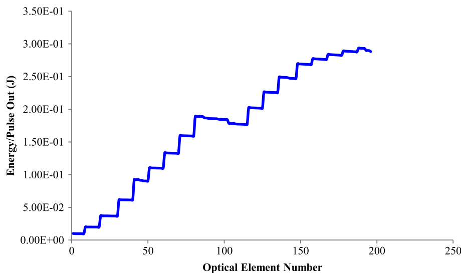
Figure 15. Evolution of the energy/pulse in Thor-300 cryogenic laser system as a function of the optical element number and at a 1 kHz repetition rate. The pump pulse duration is 500 \mu s. The Gaussian beam radius in elements 1–82 is 2 mm; after beam expansion at element 82, the beam radius is 3.5 mm.
