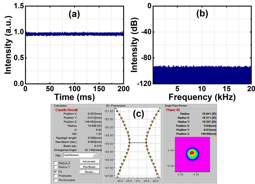
Figure 8. Output temporal property and beam quality of the signal laser at the maximum output power: (a) normalized intensity evolution; (b) corresponding power spectral density; (c) beam quality.
