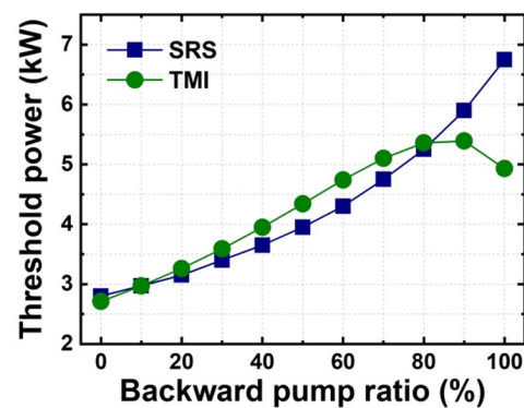
Figure 2. SRS and TMI threshold evolution along with the backward-pumped power ratio.
