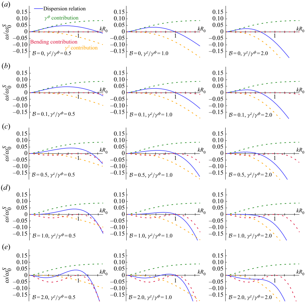
FIGURE 2. Dispersion relations for bending resistance and anisotropic interfacial tension. We distinguish the contributions from bending resistance B (red), \gamma^\phi (green) and \gamma^z (orange). From left to right the anisotropy ratio increases, whereas from top to bottom the bending resistance increases, with values given as labels. The bending and \gamma^z contributions are stabilising for all wavenumbers, while the \gamma^\phi -contribution destabilises the interface. Bending either reduces the unstable range from its right, large kR_0 , boundary (classical regime) and/or restricts the range of growing modes by the appearance of another positive root to its left, small kR_0 , boundary (restricted regime). The maximum of the dispersion relation shifts depending on bending resistance. Large bending and anisotropy in (d,e) on the right can even lead to a purely negative dispersion relation, thus completely suppressing the Rayleigh–Plateau instability (suppressed regime).
