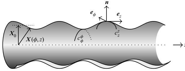
FIGURE 1. Cylindrical, elastic interface under periodic perturbation. We consider an axisymmetric interface between an inner, enclosed and an outer, surrounding fluid. The surface of the complex interface is parametrised by X(\phi, z) , the undeformed reference state (dotted line) is described by X_0 . The in-plane coordinate vectors which point along the interface are e_\phi and e_z , the unit normal vector on the interface n points outwards. In addition to the azimuthal curvature c_\phi^\phi along e_\phi the perturbation leads to an axial curvature c_z^z along e_z .
