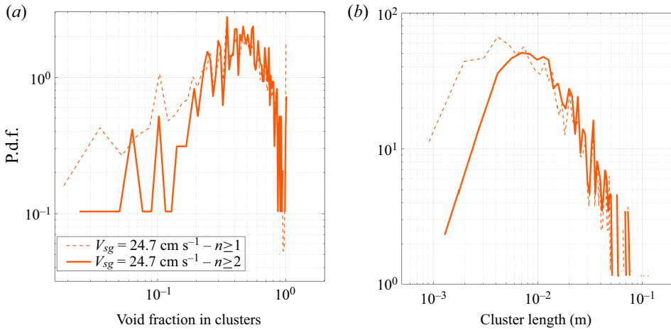
Figure 6. Comparisons of the p.d.f.s (a) of void fraction in clusters and (b) of cluster lengths when the minimum number of bubbles is set to one or to two. Measurements performed in a D = 0.4 \text{ m} column, on the column axis at H/D = 3.625 and V_{sg} = 24.7 \text{ cm s}^{-1} .
