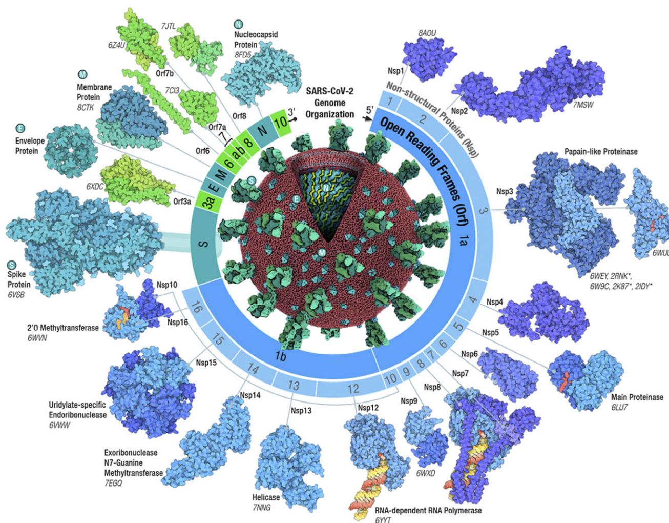
Figure 5. SARS-CoV-2 Genome and Proteome Organization. Near complete 3D knowledge of the SARS-CoV-2 proteome derives from >4,600 SARS-CoV-2 related PDB structures and CSM based on SARS-CoV-2 related structures archived in the PDB. Figure adapted from (Lubin et al. , 2022) and available from PDB-101 ( https://pdb101.rcsb.org/learn/flyers-posters-and-calendars/flyer/sars-cov-2-genome-and-proteins ). Color coding: shades of blue-non structural proteins; shades of green: structural proteins and proteins encoded by various open-reading frames; yellow/orange/red-duplex RNA; orange-S-adenosyl methionine; and shades of red-enzyme inhibitors.
