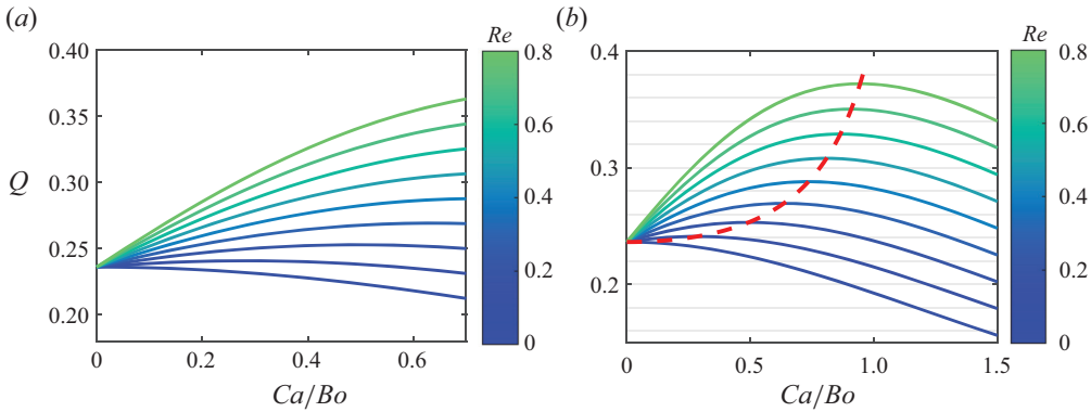
Figure 10. (a) The analytical solutions of Q plotted against Ca/Bo with different values of Re from 0 to 0.8. (b) Same asymptotic solutions with the range of Ca/Bo from 0 to 1.5, with the grey grid lines. The red dashed line depicts the maximum Q for any given Re .
