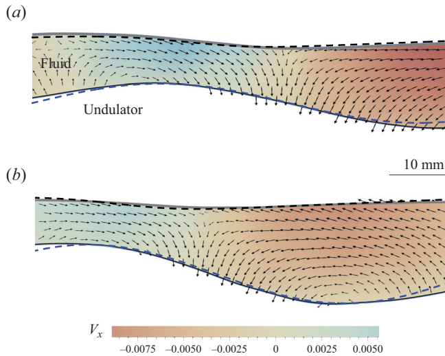
Figure 3. Results of PIV for silicone oil at V_w = 0.0177 \text{ m s}^{-1} at two different instances of time: (a) at t = 0 and (b) t = 0.48 \text{ s} . The colour coding inside the thin film represents the horizontal component of the laboratory-frame velocity field that is taken to be positive in the direction of V_w . The black and the blue dashed line are the theoretical predictions of the dimensional free surface shape and the dimensional profile of the undulating boundary with (a) h_1 = \sin(2\pi x) for x \approx 0-0.81 and (b) h_1 = \sin(2\pi x + 0.873) for x \approx 0-0.81 .
