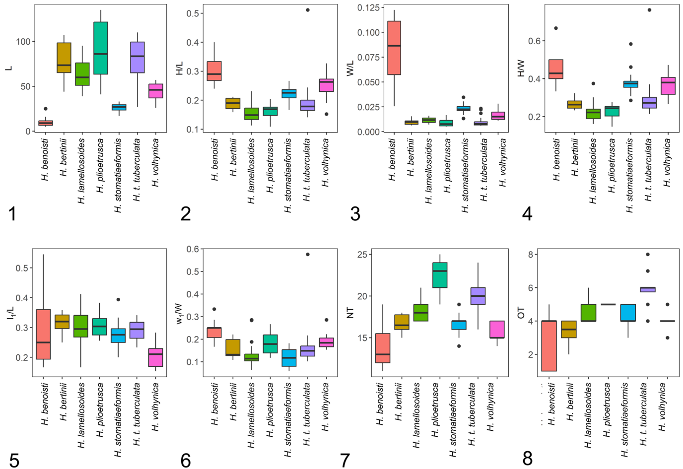
Figure 6. Box plots showing univariate comparisons among European known fossil and extant abalone species. (1) Shell length. (2) Height:length ratio. (3) Width:length ratio. (4) Height:width ratio. (5) Relative spire position with respect to L. (6) Relative spire position with respect to W. (7) Total number of tremata. (8) Open tremata. Boxes illustrate first and third quartile as box edges and median as central line.
