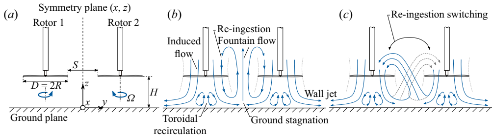
Figure 1. (a) Schematic representation of the side-by-side rotor system in ground effect with relevant parameters and system of coordinates. (b) Conceptual flow topology. (c) Illustration of re-ingestion switching.
