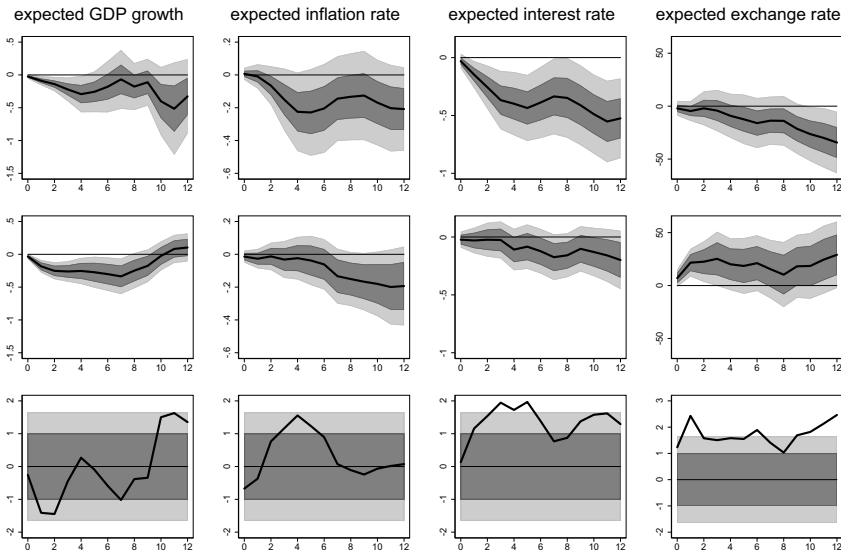
Figure A.5. Responses of expectations to global uncertainty conditional on monetary independence (GEMU). Notes: The figure shows impulse response functions of the survey measures to a one-standard deviation surge in the uncertainty measure by Baker et al. (2016). In each panel, the upper panels show responses of expected growth rates where the policy choice is evaluated at 0 and at 1 in the middle panel. The lower panels show t-statistics on the difference between responses. See also notes in Figure 2.
