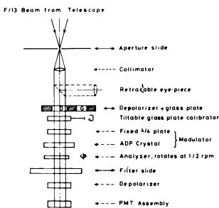
Figure 1. Optical arrangement of the polarimeter
