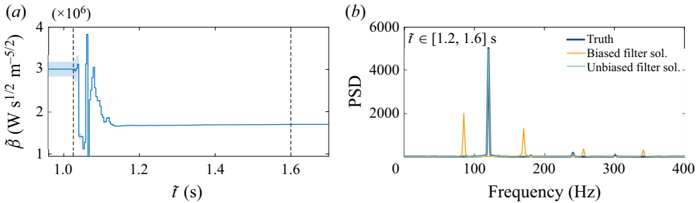
Figure 25. Real-time learning of the model bias, unbiased state and parameters. (a) Time evolution of the parameter \tilde{\beta} with the standard deviation. (b) Power spectral density (PSD) of the pressure oscillations at \tilde{x}/\tilde{L}_0 = 0.18 of the true pressure oscillations (dark blue), biased filtered solution (orange) and unbiased filtered solution (light blue). The vertical dashed lines show the assimilation window.
