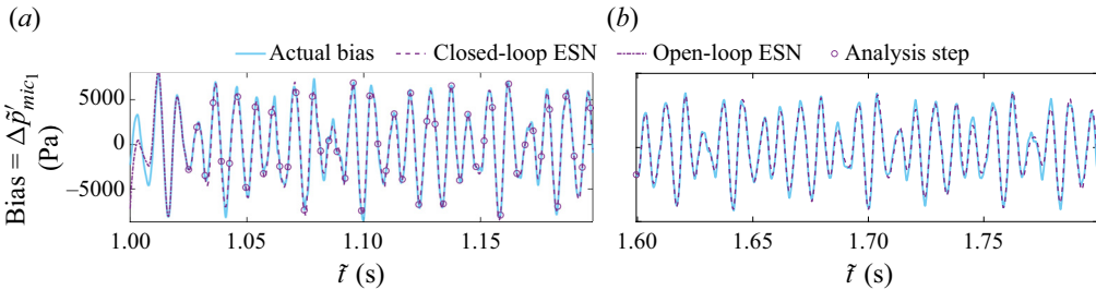
Figure 26. Real-time learning of the model bias, unbiased state and parameters. Comparison of the actual bias and the estimated model bias from the ESN during state and parameter estimation. (a) Open-loop initialisation and sequential closed loops re-initialised at analysis steps. (b) Echo state network's closed-loop forecast after data assimilation ends.
