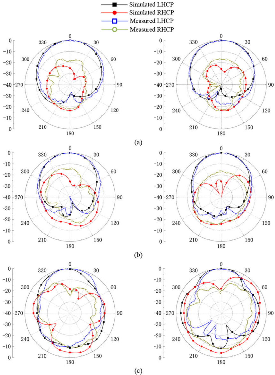
Figure 12. Normalized radiation patterns in xoz plane (left side) and yoz plane (right side), (a) at 3.75 GHz; (b) at 4.2 GHz; (c) at 4.65 GHz.
