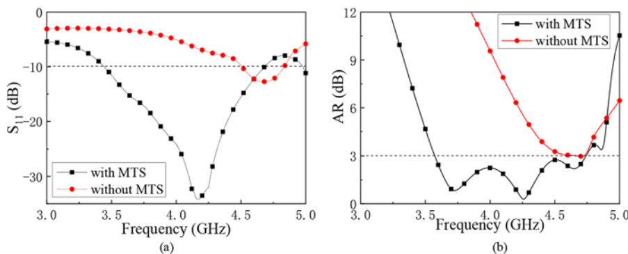
Figure 6. Simulated results of the antenna with or without the metasurface, (a) S_{11} ; (b) AR.
