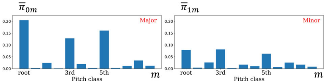
Fig. 5. The emission probabilities \bar{\pi} obtained by the tatum-level model assuming the independence of \mathbf{S} .
