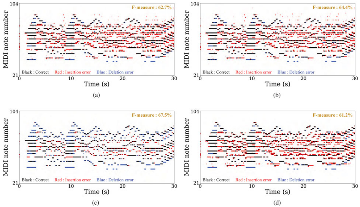
Fig. 7. Piano rolls estimated for MUS-chnp_p19_ENSTDkCl. (a) Sparse model, (b) chord-aware model ( \alpha = 1 ), (c) chord-aware model ( \alpha = 12.5 ), (d) chord-aware Markov model ( \alpha = 12.5 ).
