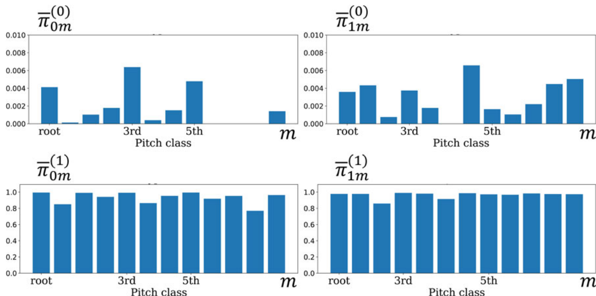
Fig. 9. The emission probabilities \bar{\pi} estimated for MUS-chpn_p19_ENSTDkCl.
