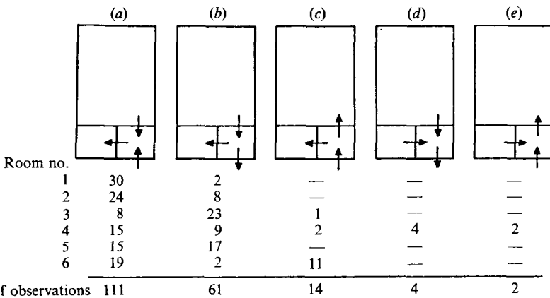
Fig. 4. Ventilation patterns observed for the patient rooms. (a), directions of air flow designed; (b), (c), (d) and (e), other observed air-flow patterns. The table shows a number of times the respective pattern was observed in the specified room.
