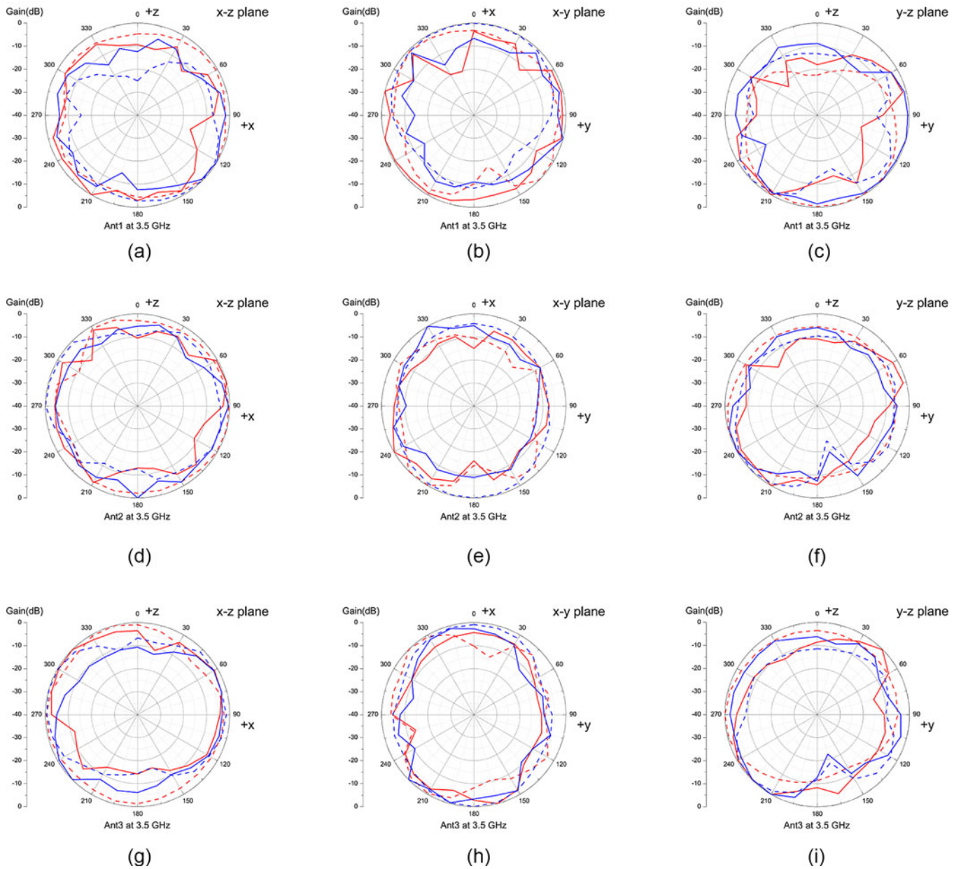
Figure 15. Simulated and measured radiation patterns for the proposed MIMO antenna at 3.5 GHz: (a) xz -plane, (b) xy -plane, and (c) yz -plane for Ant1, (d) xz -plane, (e) xy -plane, and (f) yz -plane for Ant2, and (g) xz -plane, (h) xy -plane, and (i) yz -plane for Ant3.
