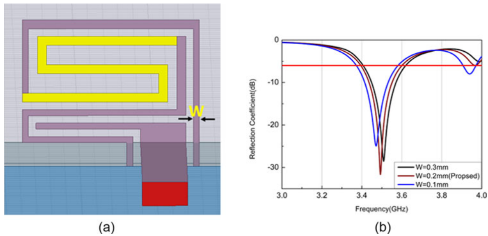
Figure 5. (a) The parameter W for the proposed antenna and (b) variation in the reflection coefficient as W varies.
