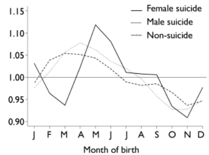
Fig. 4 Mean detrended seasonal components by gender.
