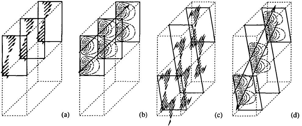
FIGURE 2. The example toroidal field of Section 3.4.3, l_y = 1 ; projection and periodicity ( k and \gamma ) as in Figure 1: (a, b) l_z = 0 ; (c, d) l_z = 1 ; (a, c) schematic of force distribution; (b, d) chain-lines mark vortex lines (which are also contours of constant velocity, by [9, Theorem 2]) and solid lines the stream-lines of maximum velocity.
