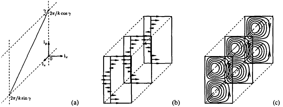
FIGURE 1. Poloidal rolls from the example in Section 3.4.2 with k = 2 , \gamma = \pi/8 , l_y = 1 , l_z = 0 and s = -1/2 : (a) geometry; (b) schematic of the force distribution; (c) stream-lines (solid) and roll axis (chain-line). Also marked in (b) and (c) are two yz -period cells and |x| = 1 (dashed) and the planes \zeta_\ell = 0 , \pi \cos \beta_\ell/k \sin \gamma and 2\pi \cos \beta_\ell/k \sin \gamma (solid).
