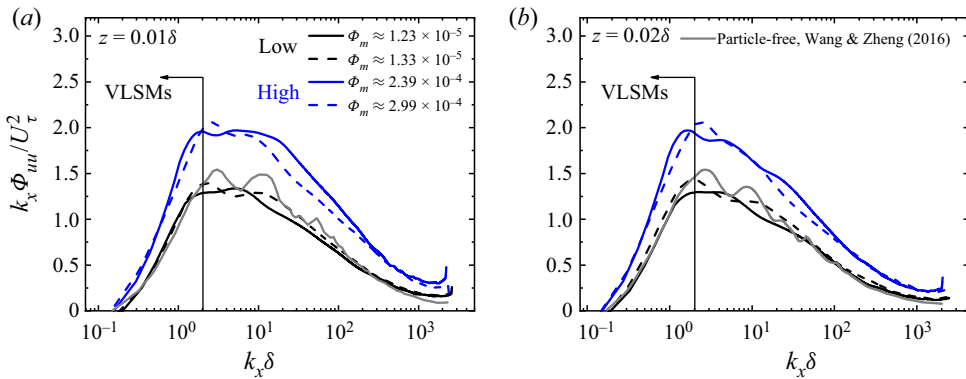
Figure 5. Pre-multiplied energy spectra of the streamwise velocity fluctuations k_x \Phi_{uuu} / U_\tau^2 vs the streamwise wavenumber k_x \delta at (a) z \approx 0.01\delta and (b) z \approx 0.02\delta from datasets with different particle mass loading: black lines, low \Phi_m (no. 1 and no. 2); blue lines, high \Phi_m (no. 11 and no. 13). The grey lines are the particle-free results in Wang & Zheng (2016).
