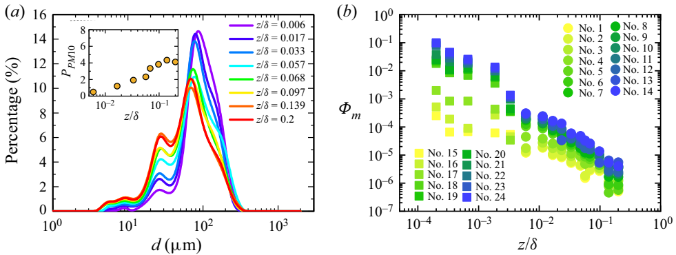
Figure 3. (a) Particle diameter distribution of the sand grains at different wall-normal locations, where the illustration shows the percentage of particles with diameters smaller than 10 μm. (b) Variation in \Phi_m with the outer-scaled wall-normal distance. It is noted that ‘No.’ refers to the sample sets in table 1.
