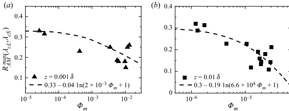
Figure 16. Variations in the amplitude modulation coefficient with the particle mass loading \Phi_m at wall-normal distances of z \approx 0.001\delta (nos. 15–24) (a) and 0.01\delta (nos. 1–14) (b). The filled symbols are the current ASL experimental results, and the lines are the fitting curves.
