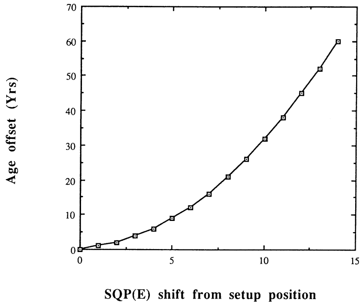
Fig. 6. Error in ^{14}\text{C} age as a function of SQP(E) if purity and gain variations are not corrected for
