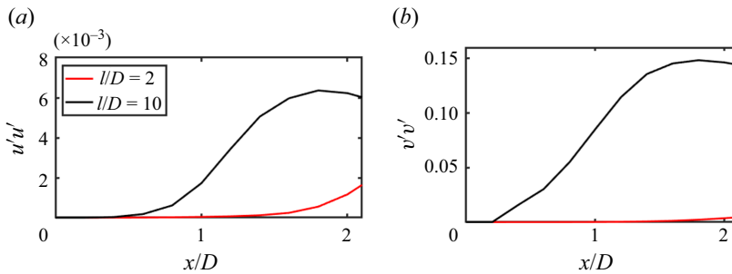
Figure 10. Distribution of velocity fluctuations along a horizontal sampling line at (y, z) = (0, 0) (a) u'u' , (b) v'v' .
