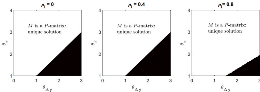
Figure 6. Regions in which M is not a P -matrix (black) for T = 16 and various \rho_i .
