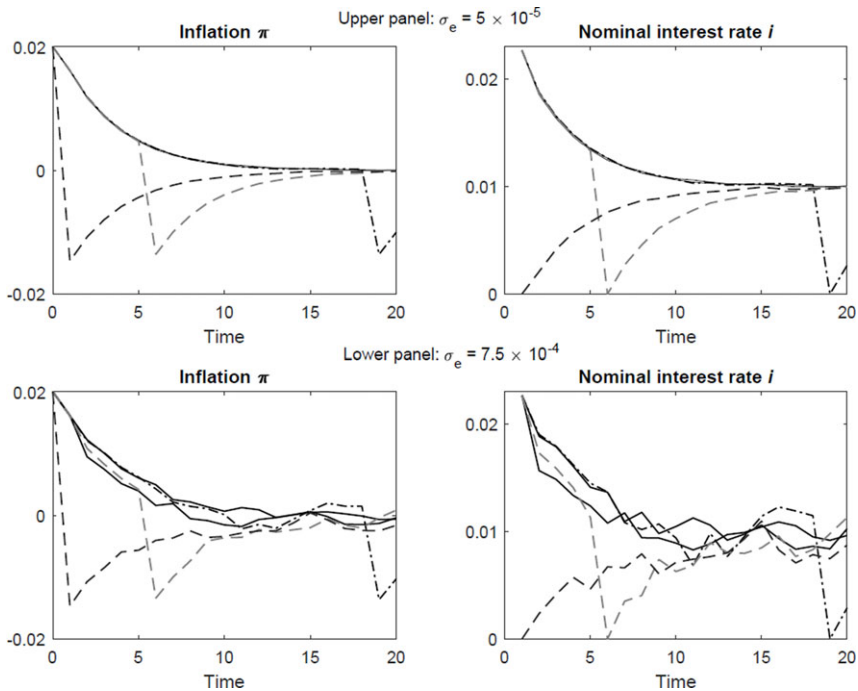
Figure 3. Five stochastic simulations: \rho_1 = 0.95 and initial values \pi_0 = 0.02, e_1, e_2 = -0.001 .
