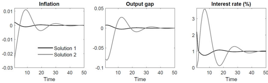
Figure 10. “Good” and “bad” solutions under price-level targeting for e_1 = 0.01 , r_0^* = y_0 = 0 and a “weak” response to the price level \theta_p = 0.015 when \sigma = 1 , \theta_{\Delta y} = 1.6 and \rho_i = 0 .
