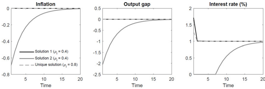
Figure 7. Perfect foresight solutions with interest rate smoothing when e_1 = 0.01, i_0^* = y_0 = 0, \sigma = 1 and \theta_\pi = 1.5, \theta_{\Delta y} = 1.6 : two different values of \rho_i ( \rho_i = 0.4 , solid; \rho_i = 0.8 , dashed).
