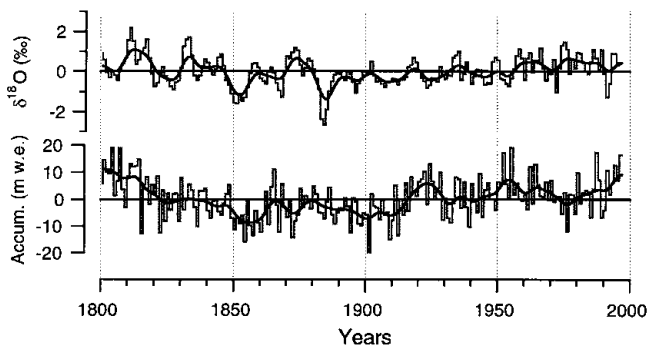
Fig. 8. Composite annually resolved time series of \delta^{18}\text{O} values (above) and accumulation rates (below). Shown are the deviations of annual values from the 1800–1997 means. The smoothed curve was calculated using a Gaussian low-pass filter over 11 years.
