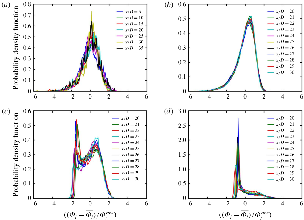
FIGURE 15. (Colour online) The probability density function of mass-weighted stream age on the scaled sample space at (a) \eta = 0 , (b) \eta = 0.08 , (c) \eta = 0.16 and (d) \eta = 0.20 .
