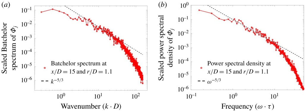
FIGURE 13. (Colour online) (a) Energy spectrum of mass-weighted stream age and (b) power spectrum by direct Fourier transform of the mass-weighted stream age at x/D = 15 and r/D = 1.1 .
