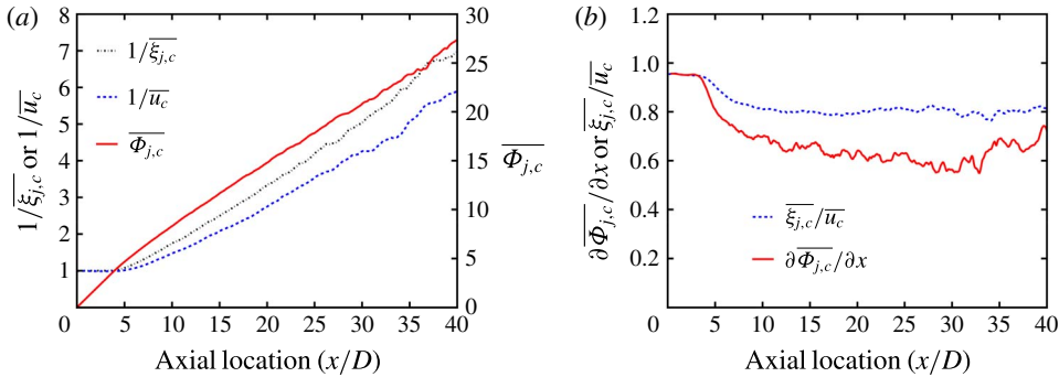
FIGURE 7. (Colour online) Axial variation of: (a) the centreline average of mass-weighted stream age \bar{\Phi}_{j,c} (right axis) and the reciprocals of the centreline average mixture fraction 1/\bar{\xi}_{j,c} and axial velocity 1/\bar{u}_c (left axis); (b) the axial gradient of \bar{\Phi}_{j,c} and the ratio of \bar{\xi}_{j,c} and \bar{u}_c along the centreline.
