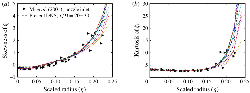
FIGURE 4. (Colour online) The skewness (a) and the kurtosis (b) of the mass fraction over the scaled radius at different axial locations.
