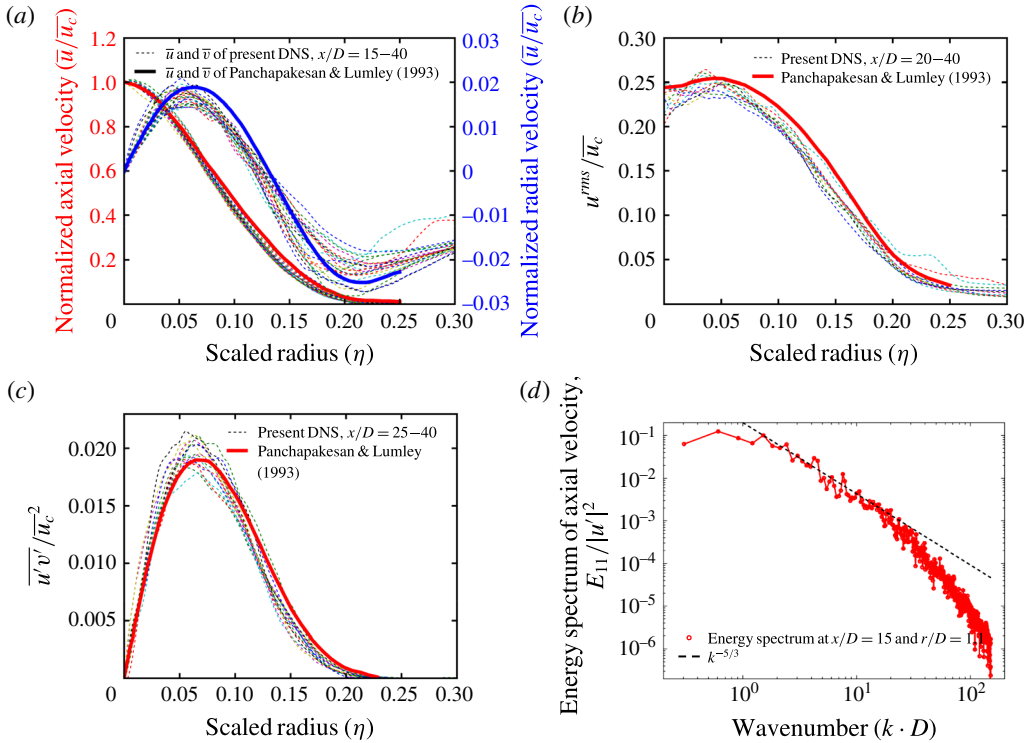
FIGURE 2. (Colour online) Radial profiles of (a) the mean axial velocity, (b) the axial velocity fluctuation, (c) the axial–radial Reynolds stress and (d) the energy spectrum of axial velocity.
