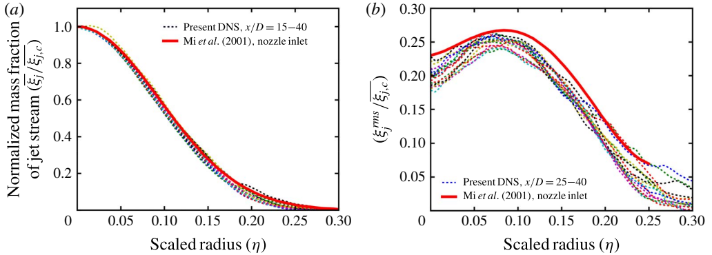
FIGURE 3. (Colour online) The radial variation of (a) the mean mass fraction and (b) the root mean square fluctuation of mass fraction.
