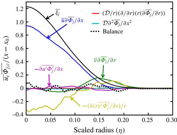
FIGURE 9. (Colour online) The budget of (3.10) versus the scaled radius. Budget terms are normalised by \bar{u}_c \Phi_{j,c} / (x - x_0) and averaged over normalised axial distances x/D = 15-40 .
