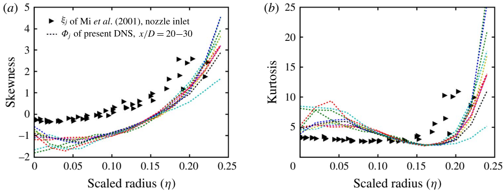
FIGURE 12. (Colour online) (a) The skewness and (b) the kurtosis of mass-weighted stream age over the scaled radius.
