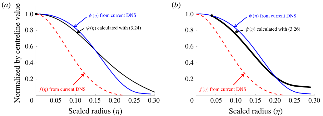
FIGURE 11. (Colour online) Comparison of the mass-weighted stream-age shape function profiles over the scaled radius between the current DNS data and solutions from (a) (3.24) and (b) (3.26). The parameters used are \beta_1 = 0.0038 , \beta_3 = 0.01 and B/(A\alpha) = 1.33 .
