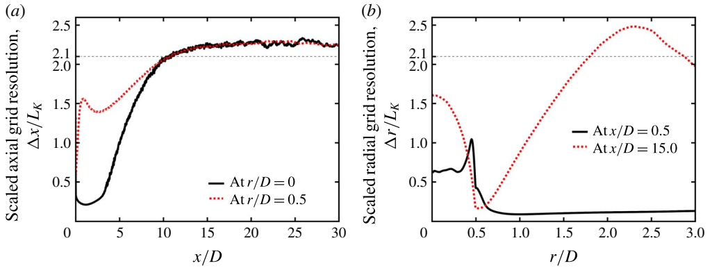
FIGURE 1. (Colour online) The ratios between the grid spacing and the calculated Kolmogorov length scale along (a) the axial direction and (b) the radial direction.
