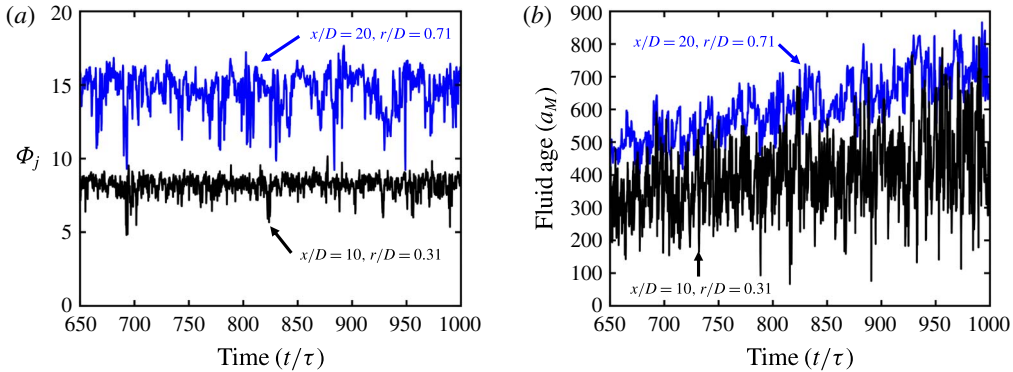
FIGURE 5. (Colour online) (a) Temporal profile of mass-weighted stream age at selected locations marked in figure 6(a,b); (b) temporal profile of fluid age at the same locations.
