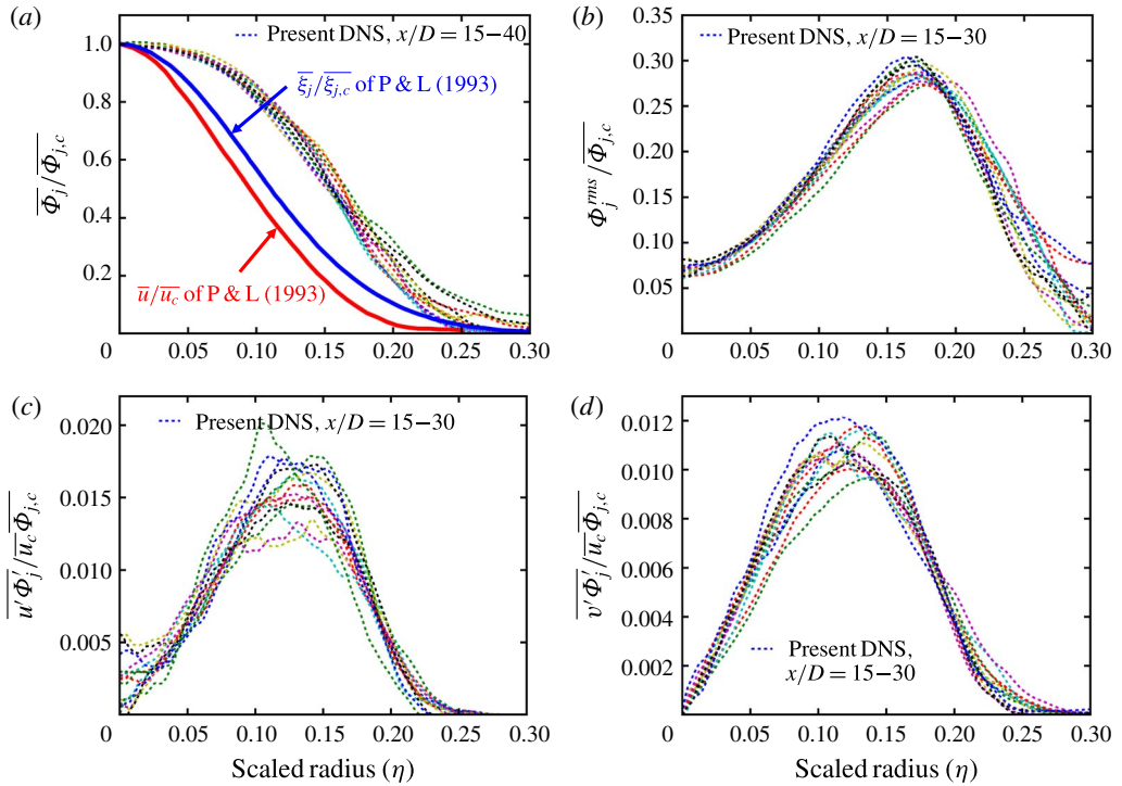
FIGURE 8. (Colour online) Radial variation of (a) the normalised mean mass-weighted stream age \overline{\Phi_j} over the range x/D = 15-40 ; (b) the normalised \Phi_j r.m.s. over the range x/D = 15-30 ; (c) the normalised axial turbulent flux \overline{u' \Phi_j} over the range x/D = 15-30 ; and (d) the normalised radial turbulent flux \overline{v' \Phi_j} over the range x/D = 15-30 .
