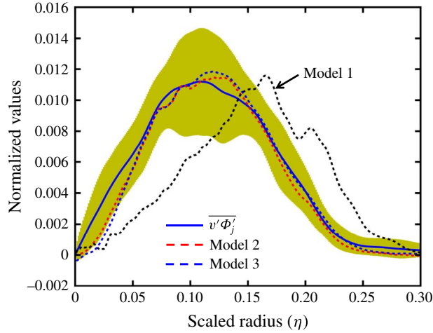
FIGURE 10. (Colour online) Comparison of the models proposed in (3.11), (3.12) and (3.15) with the DNS data of normalised radial flux of mass-weighted stream age, \overline{v'\Phi_j'}/\overline{u_c\Phi_{j,c}} (shaded area), plotted against the scaled radius, \eta . Fitting parameters are \beta_1 = 0.0015 , \beta_2 = 0.016 and \beta_3 = 0.01 .
