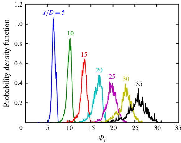
FIGURE 14. (Colour online) The probability density function of mass-weighted stream age on the centreline at axial positions in the range x/D = 5 – 35 .
