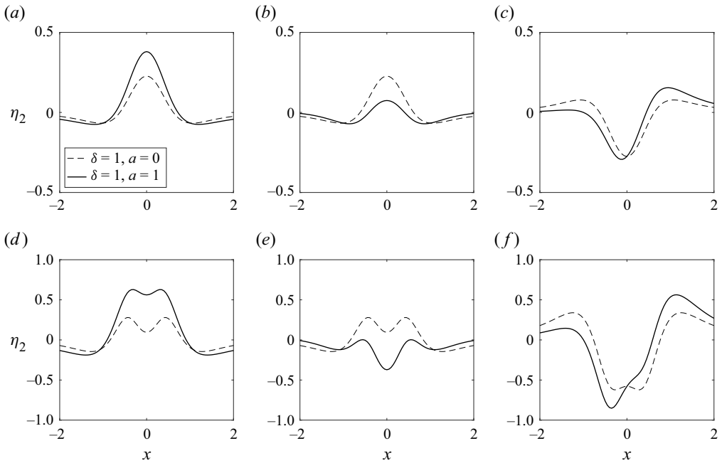
Figure 4. Second-order free surface elevation \eta_2(x) for the cylinder of non-dimensional radius ( a-c ) \varepsilon = 0.4 and ( d-f ) \varepsilon = 0.8 moving in different directions: ( a,d ) upward ( \alpha = \beta = \pi/2 ), ( b,e ) downward ( \alpha = \beta = -\pi/2 ), ( c,f ) horizontal ( \alpha = \beta = 0 ).
