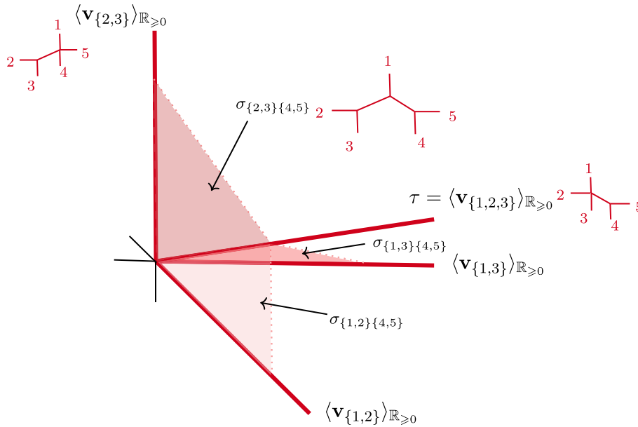
FIGURE 2. A local picture of M_{0,5}^{\text{trop}} around the ray \tau = \langle \mathbf{v}_{\{1,2,3\}} \rangle_{\mathbb{R}_{\ge 0}} . The red trees drawn next to the rays \tau , \langle \mathbf{v}_{\{2,3\}} \rangle_{\mathbb{R}_{\ge 0}} and the two dimensional cone \sigma_{\{2,3\}\{4,5\}} show the tropical curves parameterized by those cones.
