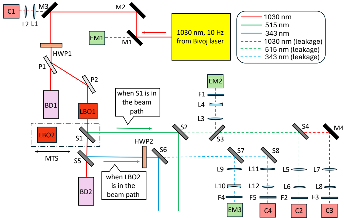
Figure 1. Experimental setup. M: mirrors; HWP: half waveplates; P: polarizers; S: harmonic separators (dichroic mirrors); L: lenses; C: cameras; EM: energy meters; BD: beam dumps; F: filters; MTS: motorized translation stage
