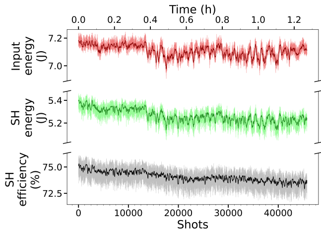
Figure 6. Long-term energy stability of the SH pulse energy. Light colored narrow lines show pulse to pulse energies whereas the darker thick lines show floating average over 100 pulses.
