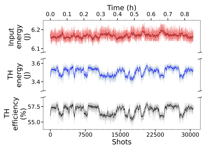
Figure 12. Long-term stability of the TH pulse energy. Light colored narrow lines show pulse to pulse energies whereas the darker thick lines show floating average over 100 pulses.
