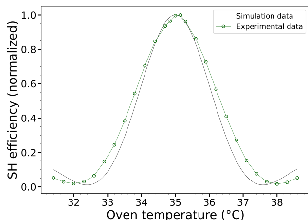
Figure 8. Dependence of the SH conversion efficiency on the oven temperature for the 20 mm long LBO crystal.
