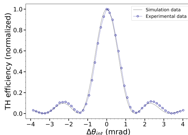
Figure 13. Dependence of the TH conversion efficiency on internal angular detuning for 20 mm long LBO crystal.
