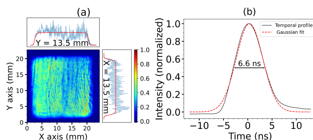
Figure 11. (a) Near-field profile of the TH beam at 3.5 J. (b) Temporal profile of the TH beam.
