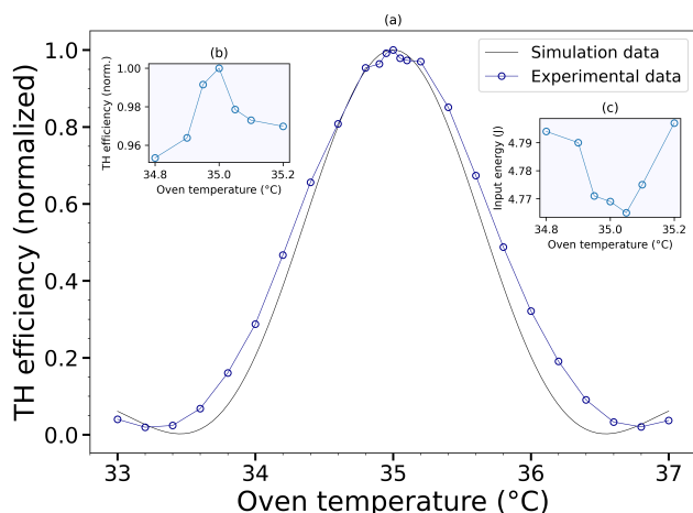
Figure 14. (a) Dependence of the TH conversion efficiency on the oven temperature for the 20 mm long LBO crystal. (b) Dependence of the TH conversion efficiency on the oven temperature with a reduced range of temperature points on the x-axis. (c) Input fundamental energy measured at the different oven temperature as it enters the crystal.
