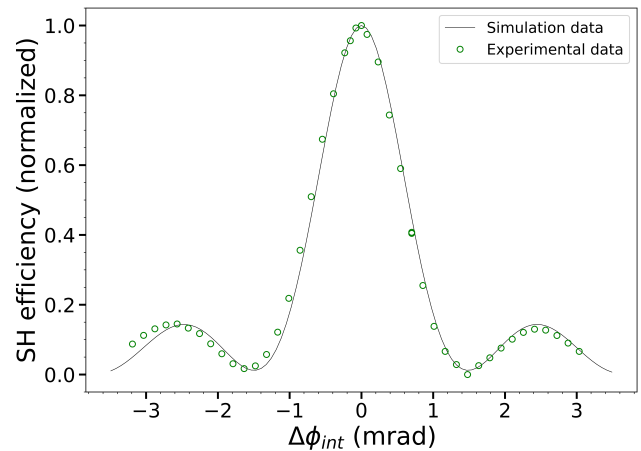
Figure 7. Dependence of the SH conversion efficiency on internal angular detuning for 20 mm long LBO crystal.
