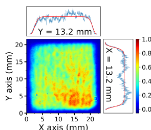
Figure 9. Near-field profile of the input fundamental beam at 6.1 J.
