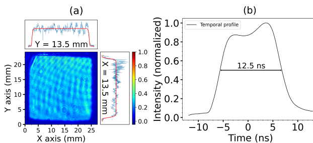
Figure 5. (a) Near-field profile of the unconverted fundamental beam. (b) Temporal profile of the unconverted fundamental beam.
