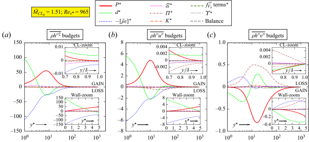
Figure 14. Budgets, at (Re_{\tau^*}, \bar{M}_{CL_x}) = (965, 1.51) , of the transport equations (6.1a) and (6.1b), for (a) \overline{\rho h''^2} , (b) \overline{\rho h'' u''} and (c) \overline{\rho h'' v''} , in (\cdot)^* units, plotted against y^* (log scale), with wall-zoom (against y^* , linear) and centreline-zoom (against y/\delta , linear), from the present DNS database (table 1).
