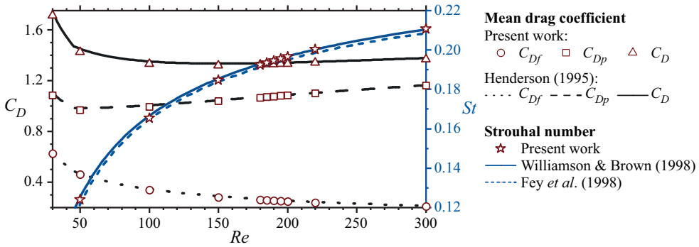
Figure 12. Comparison of mean pressure \overline{C_{Dp}} , friction \overline{C_{Df}} and total \overline{C_D} drag coefficients and Strouhal number St with the fitting curves by Henderson (1995), Williamson & Brown (1998), and Fey et al. (1998) for the two-dimensional base flow at 30 \leq Re \leq 300 .
