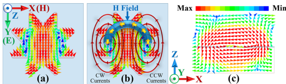
Figure 6. (a) Surface current distribution at 10.72 GHz, (b) illustration of magnetic field generation due to the counterclockwise (CCW) and clockwise (CW) current loops, and (c) magnetic field distribution at 10.72 GHz.
