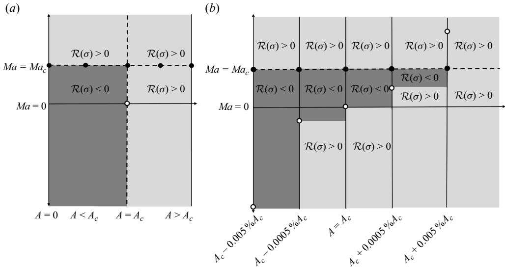
Figure 6. Illustration of Ma versus A depicting the sign of the real part of \sigma , \mathcal{R}(\sigma) for the short-wave regime. The symbol • represents Ma_s and the symbol ○ represents Ma_o . The dark region represents \mathcal{R}(\sigma) < 0 and the light region represents \mathcal{R}(\sigma) > 0 .
