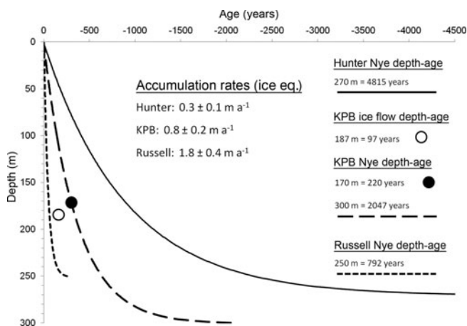
Fig. 11. Depth-age estimates for MH, KPB and MR, calculated from models developed by Nye (1953) and Haefeli (1961). The black dot at 170 m depth represents the depth of SCS overlying complex strata imaged with GPR in KPB. The open circle represents depth and age of SCS calculated from our flow model.
