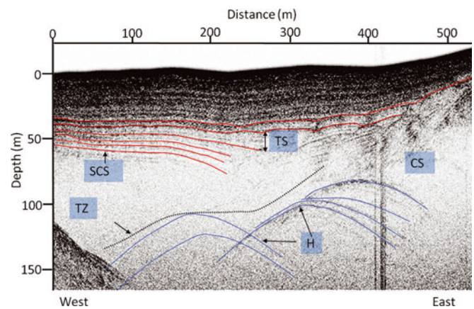
Fig. 8. Zoom of 100MHz GPR profile between A and A' (Fig. 12) from KPB. Image shows interpreted transition zone (TZ) between surface-conformable strata (SCS) and complex strata (CS). Thickening strata (TS) from compression, and relic avalanche debris in the form of hyperbolic events (H) are also visible.
