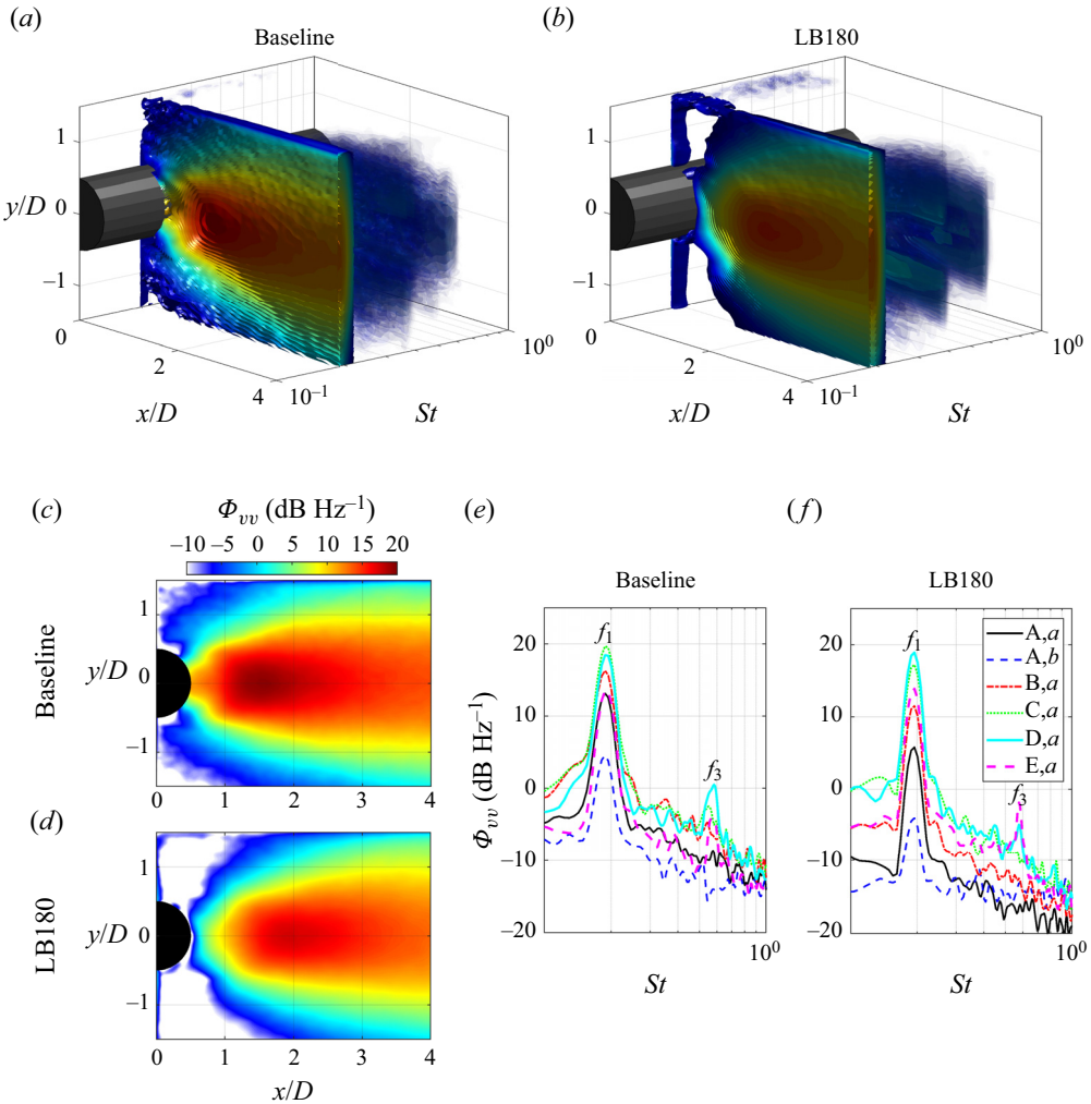
Figure 18. Isosurface of the y -component of velocity PSD, \Phi_{vv} = 10 \log_{10} \phi_{vv} (dB Hz ^{-1} , ref 1 m s ^{-1} ), at C_{\mu} = 0.007 . (a,b) Arbitrary 3-D view, (c,d) the \Phi_{vv} at the f_1 -tone frequency and (e,f) the \Phi_{vv} values along a ( y/D = 0 ) and b ( y/D = 0.5 ) for stations A ( x/D = 0.7 ), B ( x/D = 1 ), C ( x/D = 1.5 ), D ( x/D = 2 ) and E ( x/D = 4.5 ).
