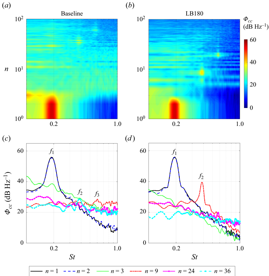
Figure 24. The PSD of temporal mode coefficient, \Phi_{cc} = 10 \log_{10} \phi_{cc} (dB Hz -1 , ref 1), shown as a function of St and mode order, n , at C_\mu = 0.007 . The f_1, f_2 and f_3 correspond to the fundamental vortex-shedding tone (first harmonic), second harmonic and third harmonic, respectively.
