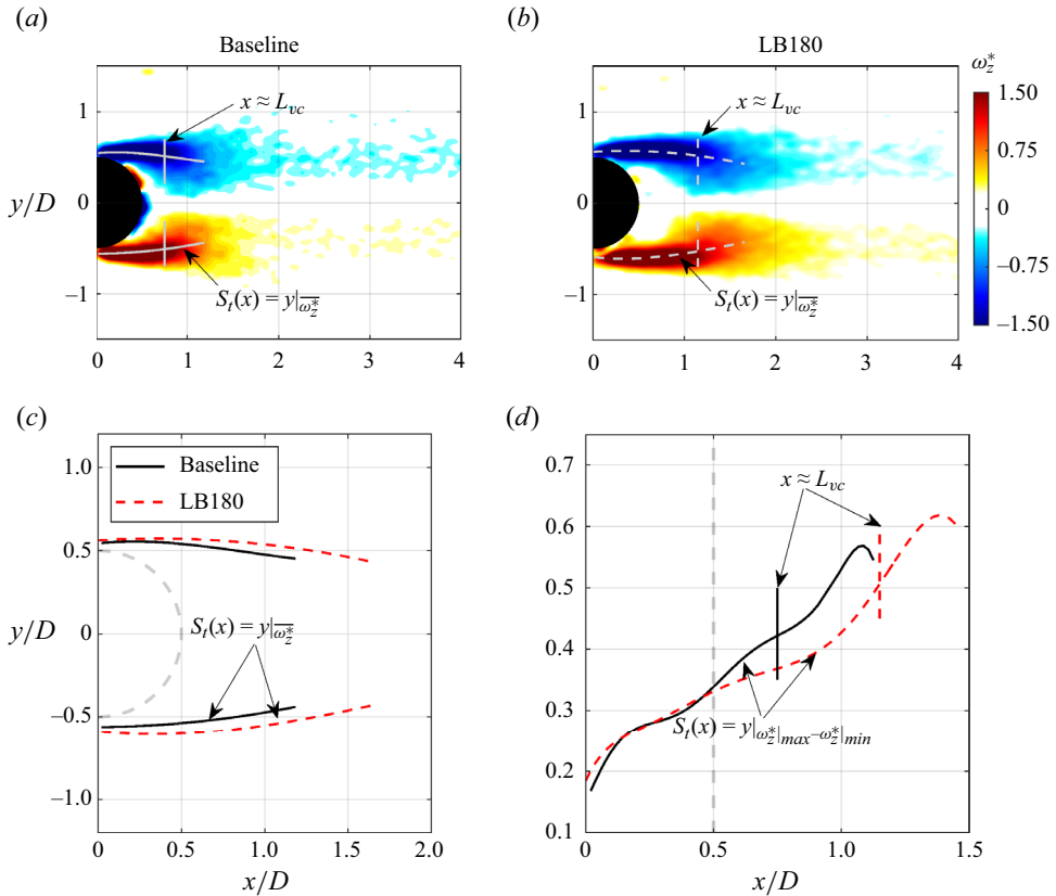
Figure 15. (a,b) Normalised time-averaged vorticity, \omega_z^* = \bar{\omega}_z D / U_\infty , superimposed by the mean shear layer trajectory, S_T(x) = y|_{\omega_z^*} , at C_\mu = 0.007 . The mean shear layer trajectory coming from the top and bottom sides of the cylinder is calculated based on \omega_z^* \leq -0.75 and \omega_z^* \geq 0.75 , respectively. Here, (c) S_T(x) = y|_{\omega_z^*} and (d) the thickness of the shear layer coming from the top side of the cylinder, S_T(x) = y|_{\omega_z^*|_{max} - \omega_z^*|_{min}} . The vertical solid and dashed lines represent x \approx L_{vc} for the baseline and LB180, respectively.
