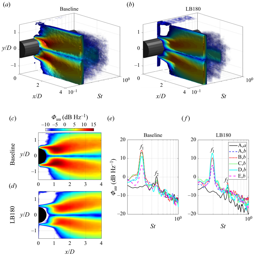
Figure 17. Isosurface of the x -component of velocity PSD, \Phi_{uu} = 10 \log_{10} \phi_{uu} (dB Hz ^{-1} , ref 1 m s ^{-1} ), at C_{\mu} = 0.007 . (a,b) Arbitrary 3-D view, (c,d) the \Phi_{uu} at the f_1 -tone frequency and (e,f) the \Phi_{uu} values along a ( y/D = 0 ) and b ( y/D = 0.5 ) for stations A ( x/D = 0.7 ), B ( x/D = 1 ), C ( x/D = 1.5 ), D ( x/D = 2 ) and E ( x/D = 4.5 ).
