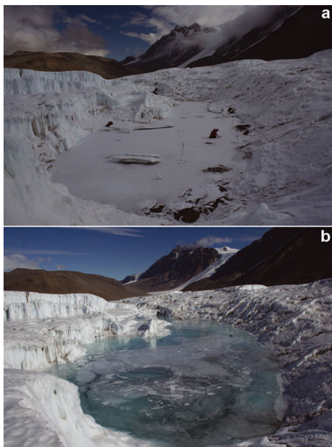
Fig. 1. A typical cryolake on the surface of Canada Glacier, Taylor Valley ( 77.61924^\circ \text{ N} , 162.96803^\circ \text{ E} ), (a) before (7 December) and (b) after (10 December) the flood event in 2008. Note the person on the lake ice in (a) for scale; the ice lid rose by 2 m in <24 \text{ hours} .
