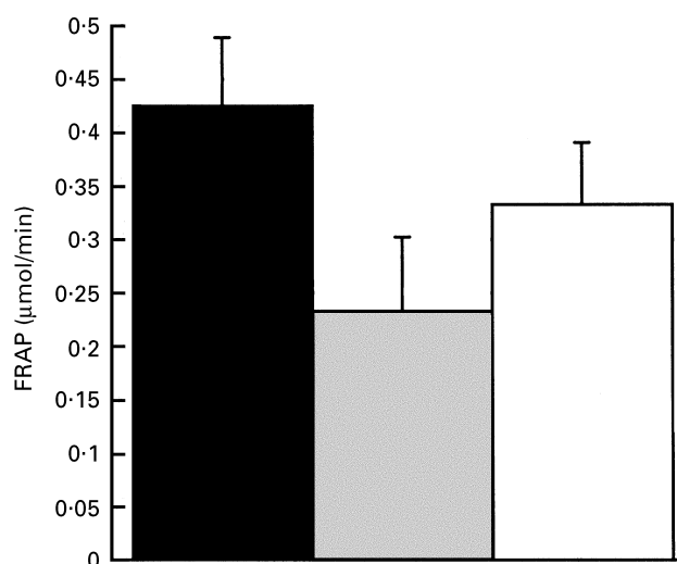
Fig. 3. Relationship between antioxidant capacity (ferric reducing ability of plasma; FRAP) and periodontal score. (■), Periodontal score of 1-12, extensive disease; (▒), periodontal score of 13-20, moderate disease; (□), periodontal score of 21-24, little or no disease. Values are means with their standard errors represented by vertical bars. For details of procedures, see Table 1 and p.140.
