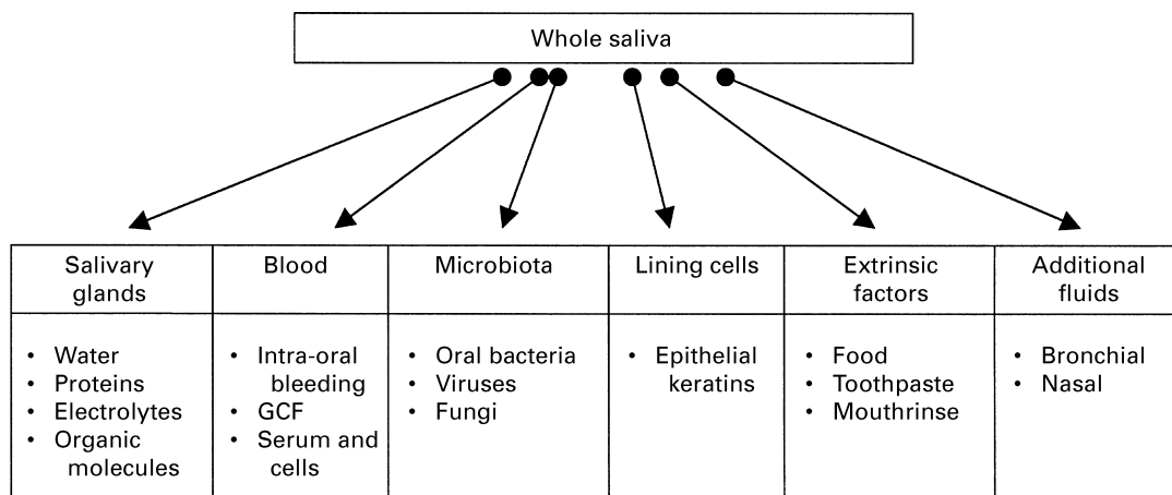
Fig. 2. Components of whole saliva. GCF, gingival crevicular fluid. (Adapted from Kaufman & Lamster, 2000.)
