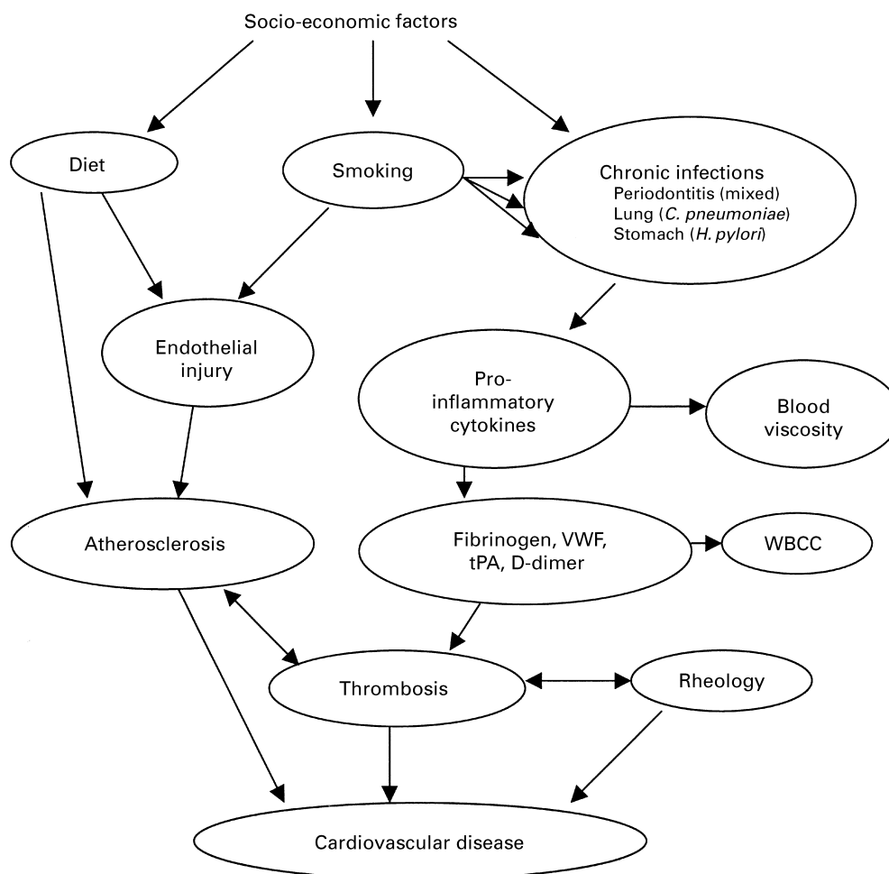
Fig. 1. Cardiovascular risk factors. C. pneumoniae , Chlamydia pneumoniae ; H. pylori , Helicobacter pylori ; VWF, von Willebrand factor; tPA, tissue plasminogen factor; D-dimer, fibrin D-dimer; WBCC, leucocyte count. (Adapted from Kinane & Lowe, 2000.)
