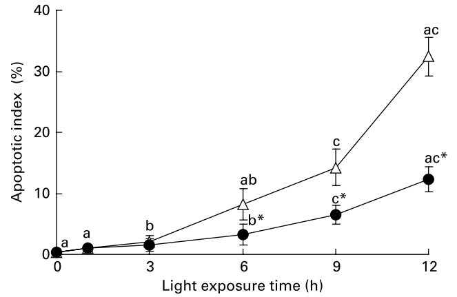
Fig. 4. Apoptotic index in the retinas of rats treated with (●) or without (○) 4% taurine for 15 d and exposed to light for 0–12 h. Values are means for six rats for each time point, with standard deviations represented by vertical bars. a,b,c Mean values with unlike letters on the same curve at different exposure times were significantly different ( P < 0.05 ; Ryan's multiple-range test). * Mean value was significantly different from that for rats at the same light exposure time treated without taurine ( P < 0.05 ; Student's t test).
