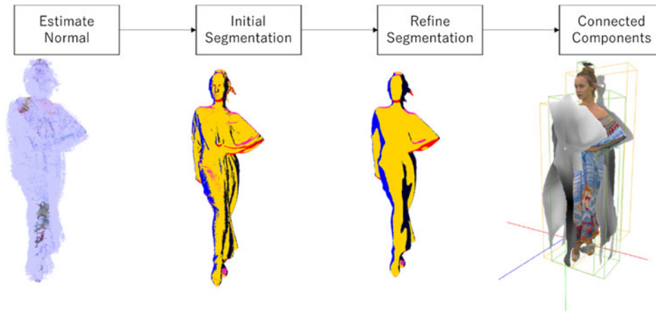
Fig. 5. Patch generation.
