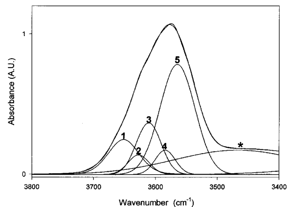
Figure 8. Deconvolution of the unaltered SWa-1 IR spectrum into several components (see Table 4) in the OH-stretching range; experimental and calculated curves.
