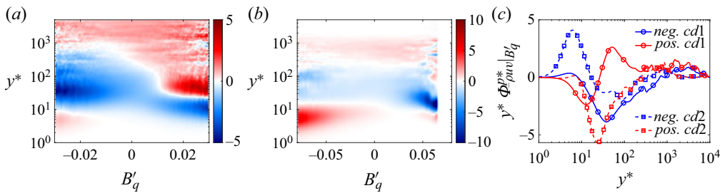
Figure 14. (a,b) Map of the conditional average of pre-multiplied velocity-pressure-gradient correlation, y^* \Phi^P_{-\rho v} |_{B'_q} , for cases (a) cold1 and (b) cold2 . (c) Profiles of the averaged y^* \Phi^P_{-\rho uv} conditioned on the extreme 2% negative and positive B'_q -events.
