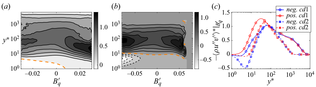
Figure 7. (a,b) Map of the conditional average of Reynolds shear stress, -\langle\rho u''v''\rangle^*|B'_q , for cases (a) cold1 and (b) cold2 . (c) Profiles of the averaged Reynolds shear stress conditioned on the extreme 2% negative and positive B'_q -events. The black solid lines in panels (a,b) denote the positive level, the black dashed lines denote the negative and the orange dashed line denotes 0.
