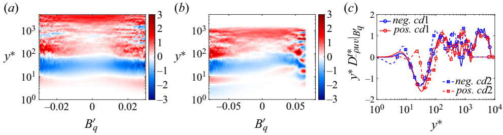
Figure 15. (a,b) Map of the conditional average of pre-multiplied turbulent diffusion of Reynolds shear stress, y^* D_{-\rho uv}^* | B'_q , for cases (a) cold1 and (b) cold2 . (c) Profiles of the averaged y^* D_{-\rho uv}^* conditioned on the extreme 2% negative and positive B'_q -events.
