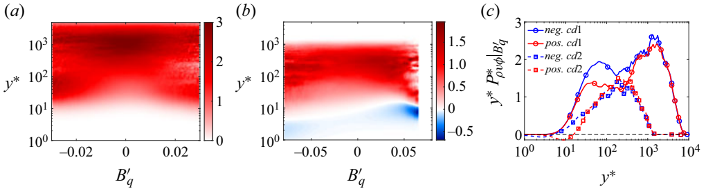
Figure 17. (a,b) Map of the conditional average of pre-multiplied turbulent-heat-flux production, y^*P_{\rho v\phi}^*|B'_q , for cases (a) cold1 and (b) cold2 . (c) Profiles of the averaged y^*P_{\rho v\phi}^* conditioned on the extreme 2% negative and positive B'_q -events. The black dashed line in panel (c) denotes 0.
