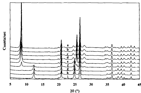
Figure 1. XRD patterns of kaolinite intercalated with hydrazine and exposed to air for (a) 0.0 h, (b) 0.5 h, (c) 3 h, (d) 4.5 h, (e) 22 h, (f) 50 h, (g) 120 h, (h) 168 h, and (i) 30 d.
