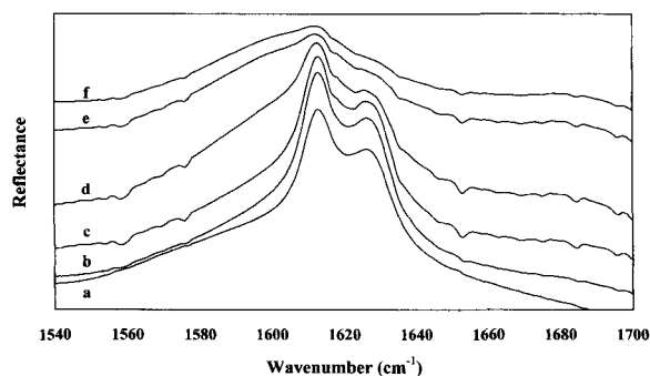
Figure 8. DRIFT spectra of the water-bending region of kaolinite intercalated with hydrazine and exposed to air for (a) 0.0 h, (b) 0.5 h, (c) 3 h, (d) 4.5 h, (e) 22 h, and (f) 50 h.
