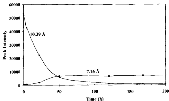
Figure 2. Relationship between the areas of the d(001) peaks of the intercalated and deintercalated-hydrazine complex as a function of time.
