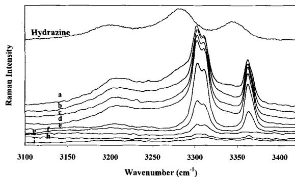
Figure 6. Raman spectra of the amine-stretching region of kaolinite intercalated with hydrazine and exposed to air for (a) 0 min, (b) 30 min, (c) 60 min, (d) 105 min, (e) 150 min, (f) 220 min, (g) 300 min, (h) 480 min, and (i) 600 min.
