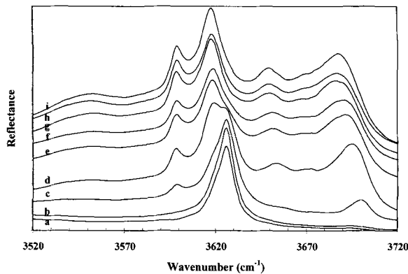
Figure 3. DRIFT spectra of the hydroxyl-stretching region of kaolinite intercalated with hydrazine and exposed to air for (a) 0.0 h, (b) 0.5 h, (c) 3 h, (d) 4.5 h, (e) 22 h, (f) 50 h, (g) 120 h, (h) 168 h, and (i) 30 d.
