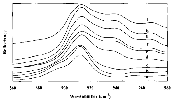
Figure 7. DRIFT spectra of the hydroxyl-deformation region of kaolinite intercalated with hydrazine and exposed to air for (a) 0.0 h, (b) 0.5 h, (c) 3 h, (d) 4.5 h, (e) 22 h, (f) 50 h, (g) 120 h, (h) 168 h, and (i) 30 d.
