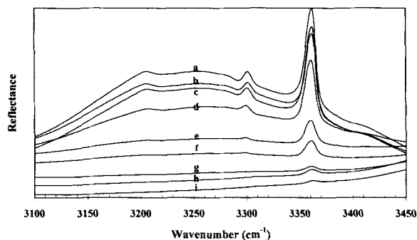
Figure 5. DRIFT spectra of the amine-stretching region of kaolinite intercalated with hydrazine and exposed to air for (a) 0.0 h, (b) 0.5 h, (c) 3 h, (d) 4.5 h, (e) 22 h, (f) 50 h, (g) 120 h, (h) 168 h, and (i) 30 d.
