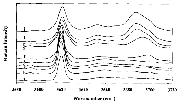
Figure 4. Raman spectra of the hydroxyl-stretching region of kaolinite intercalated with hydrazine and exposed to air for (a) 0.0 min, (b) 30 min, (c) 60 min, (d) 105 min, (e) 150 min, (f) 220 min, (g) 300 min, (h) 480 min, (i) 10 hr, and (j) 24 h.
