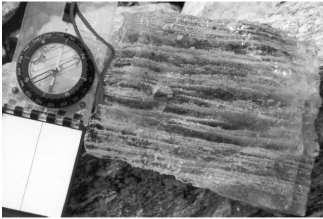
Fig. 6. Close-up view of ice removed from part of foliation-rich dark band exposed at surface of glacier, next to crevasses on western margin of the glacier. The ice is finely stratified, with sand and silt in between each layer. In middle-left section of ice sample is an in situ sub-rounded pebble.
