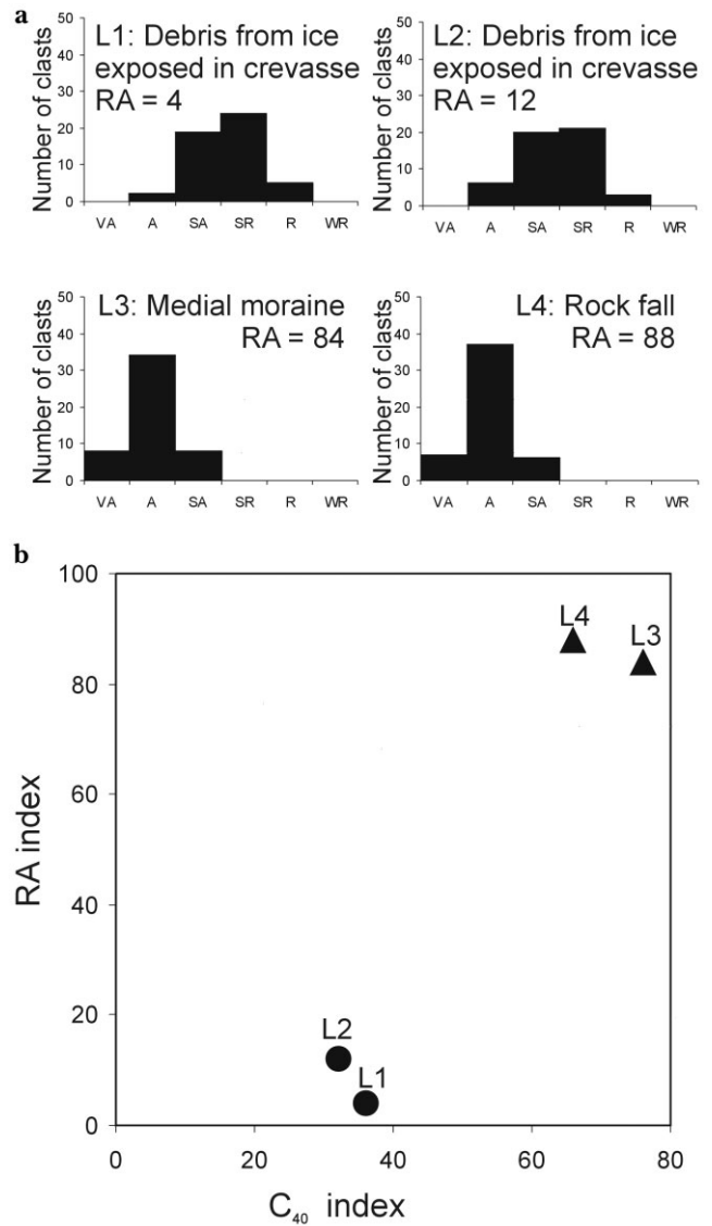
Fig. 5. (a) Clast-roundness data and (b) RA/C 40 plot for four sets of 50 clasts taken from glacier. L1 and L2 are from debris-rich foliation-parallel ice exposed in a dark ogive band by crevasse on western margin of the glacier, L3 is from a medial moraine exposed in central part of glacier and L4 is from 1995 rock fall on central part of glacier. Sample locations are shown in Figure 1b, as L1–L4.
