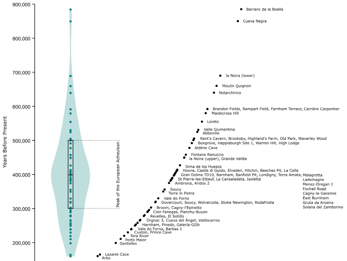
Figure 2. Temporal placement of archaeological sites in the European Acheulean record. The 'peak of the European Acheulean' is defined by the 25% and 75% quartiles across all site central dates.
