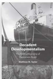
Decadent Developmentalism
